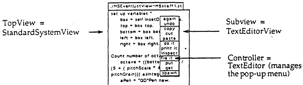
Figure 8. File-based TextEditorView and Menus
