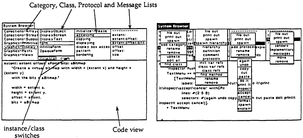
Figure 11. System Browser view layout and browser menus
