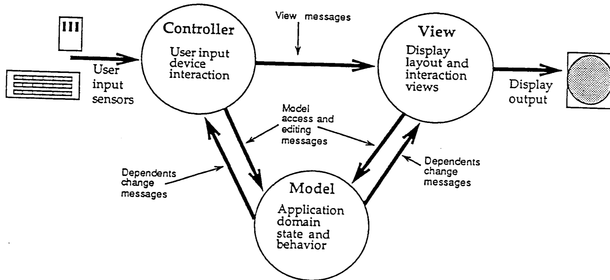
Figure 1: Model-View-Controller State and Message Sending
