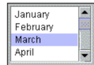
JList
