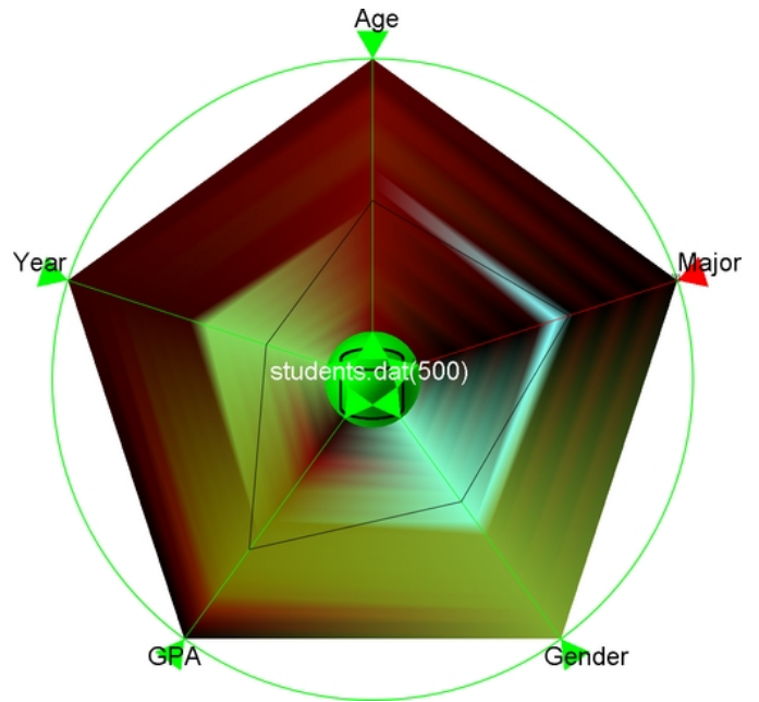
Fig. 11. Color histogram representation of a multidimensional university student dataset in a starplot visualization from the DataMeadow [29, 30]. Brightness indicates high density.
