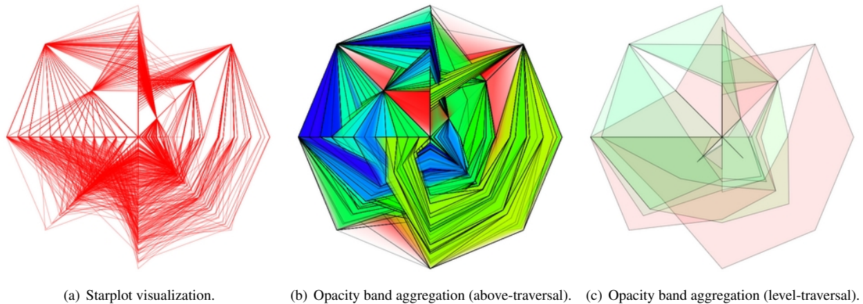
Fig. 10. Starplot visualization of an 8-dimensional dataset with opacity band [34] visual aggregations. Transparency indicates the extents and the averages for each opacity band.
