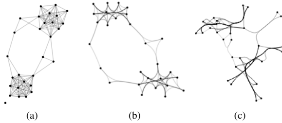
Fig. 8. Clusters in functional brain connectivity: (a) node-link diagram with force-directed layout, (b) node-link with edge bundling, (c) CD.
