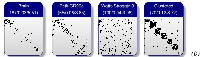
Anti-Robinson Simulated Annealing [BKS08]
