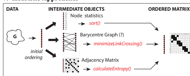
Figure 11: Heuristic Approaches for Matrix Reordering.
