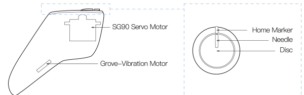
Figure 2: Design and implementation of the Tactile Device
