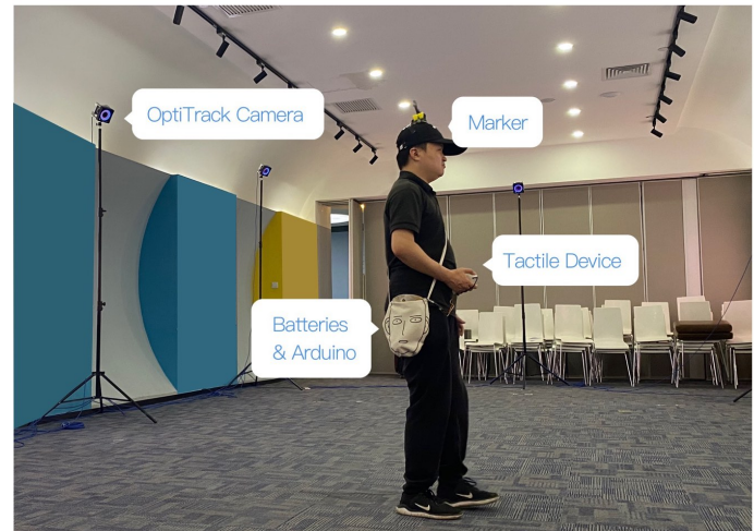
Figure 4: Apparatus and experimental setup
