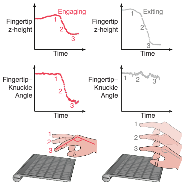
Figure 9: During engagement gesture (left), users flex their finger, causing the knuckle angle to change over time. During exiting movements (right), users did not change their knuckle angle. This difference in the movement profile can be used to identify the user's intention.
