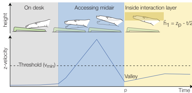
Figure 11: User’s action while accessing a midair layer and the corresponding velocity profile. Dynamic height ( \hat{h}_1 ) of the layer is set at the velocity valley, at time p .
