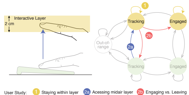
Figure 1: Interacting within an above-surface layer. We applied Buxton's three state model to explain the relevance of the user studies for such interactions.
