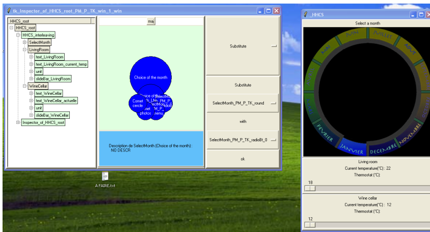
Figure 4. Choosing an alternate presentation (the round one for the ‘Select a month’ comet) in the conceptual representation. The external representation is updated accordingly.
