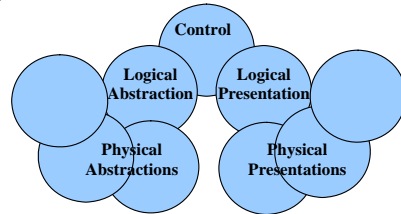
Figure 2. A comet, a software architecture construct made of a control, a logical abstraction and a logical presentation in charge of dealing with their potentially multiple physical abstractions and/or presentations. This ‘polymorphism’ may be useful for adapting to the context of use.
