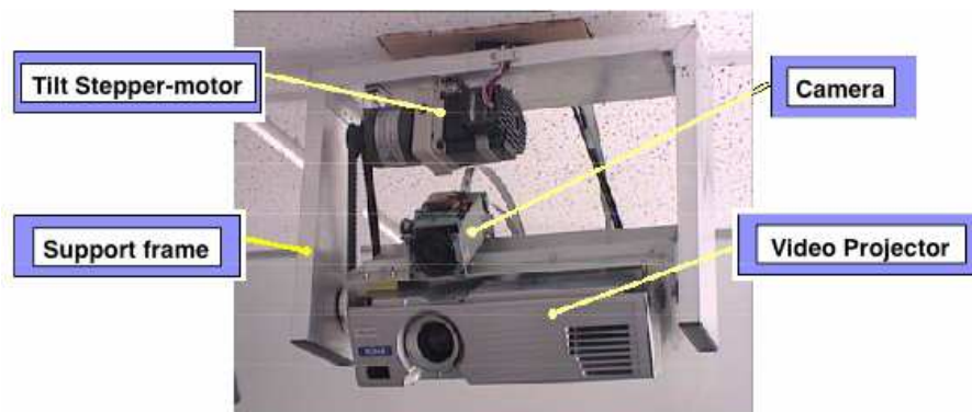
Figure 6. Le SCP (Steerable Camera-Projector)
