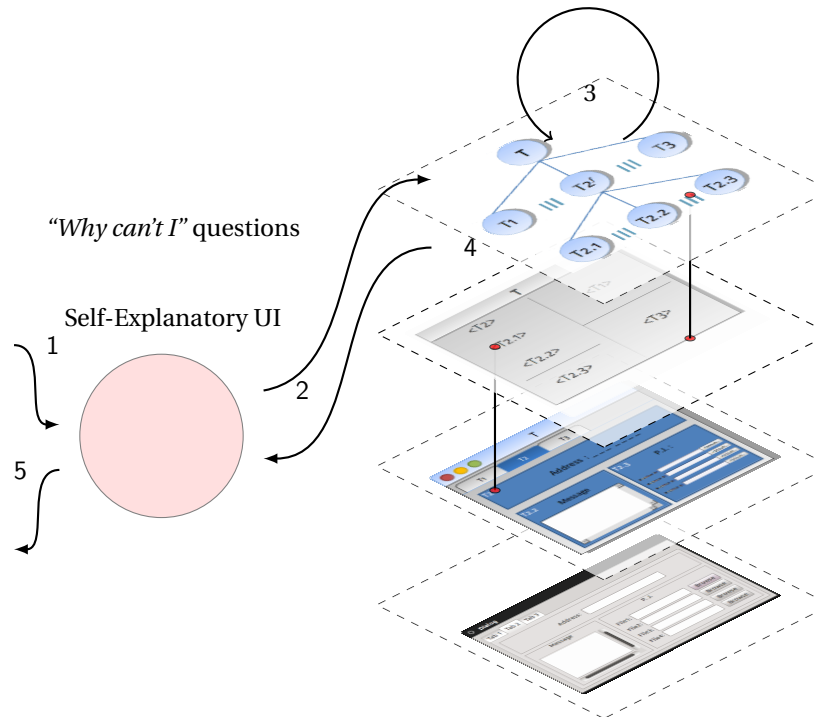
Figure 4.32: Explanation strategy for “ Why I can’t ” questions. Questions of type Behavioural are treated (1) by the explanation strategy by locating the disabled task inside the task model (2). The algorithm for finding the LOTOS operator that activates this task is then applied (3). This information is recovered by the explanation strategy (4) and the help facility uses it to compose the final answer (5).
