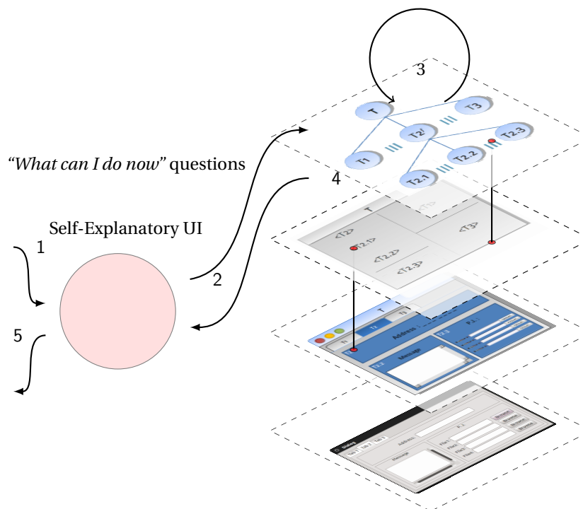
Figure 4.28: Explanation strategy for “ What can I do now ” questions. The question is identified as of type Availability by the help facility in (1). The explanation strategy locates the current active task inside the task model (2). The algorithm for finding all the currently available tasks is then applied (3). The list of available tasks is recovered by the explanation strategy in (4). Finally, the help facility composes the final answer (5).
