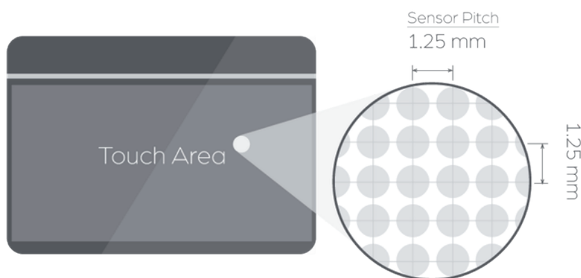
FIGURE A.16 – Sensel Morph
